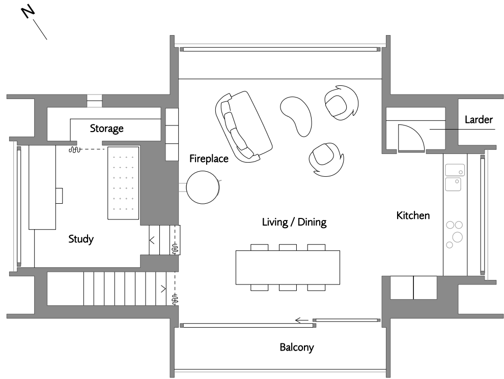
Unterhus, Second Floor Scale 1:100
