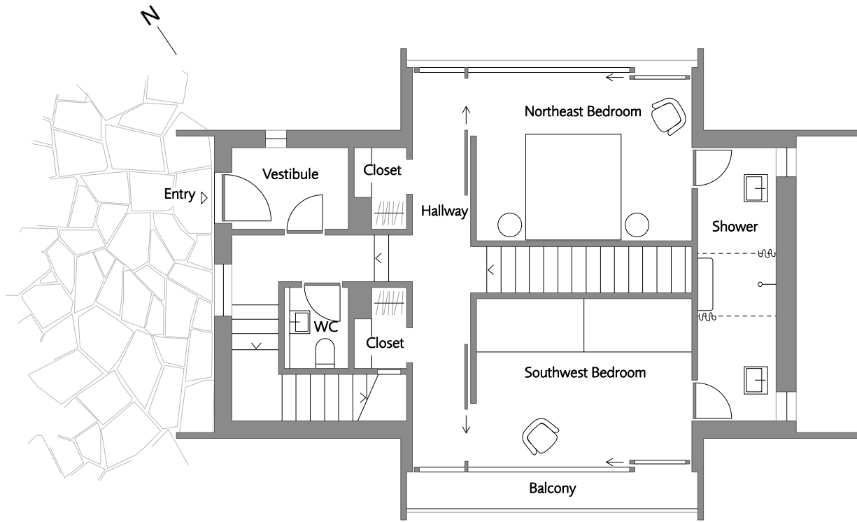
Unterhus, First Floor Scale 1:100
