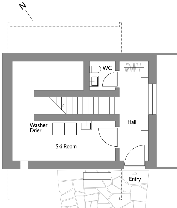
Unterhus, Ground Floor Scale 1:100
