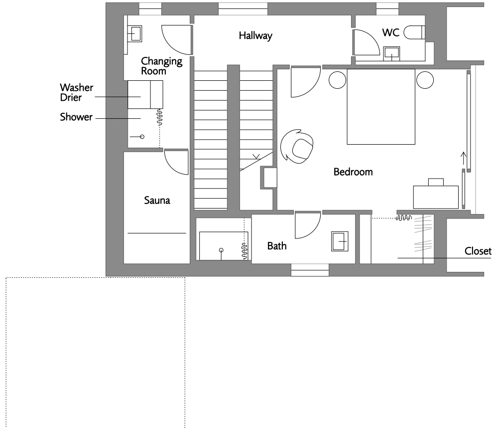
Türmlihus, First Floor Scale 1:100
